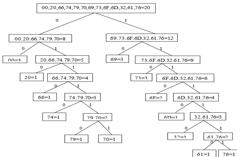
Gambar 3. Pohon Huffman
