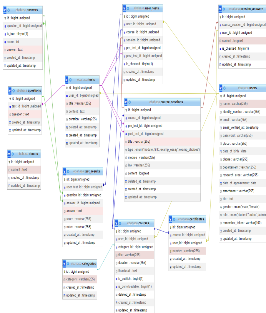
Figure 5. Database View in MySQL
